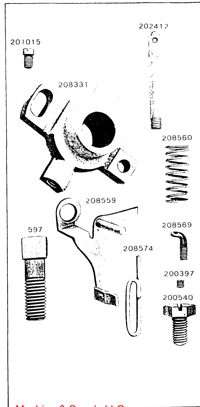
PLATE 11675--FULL SIZE
