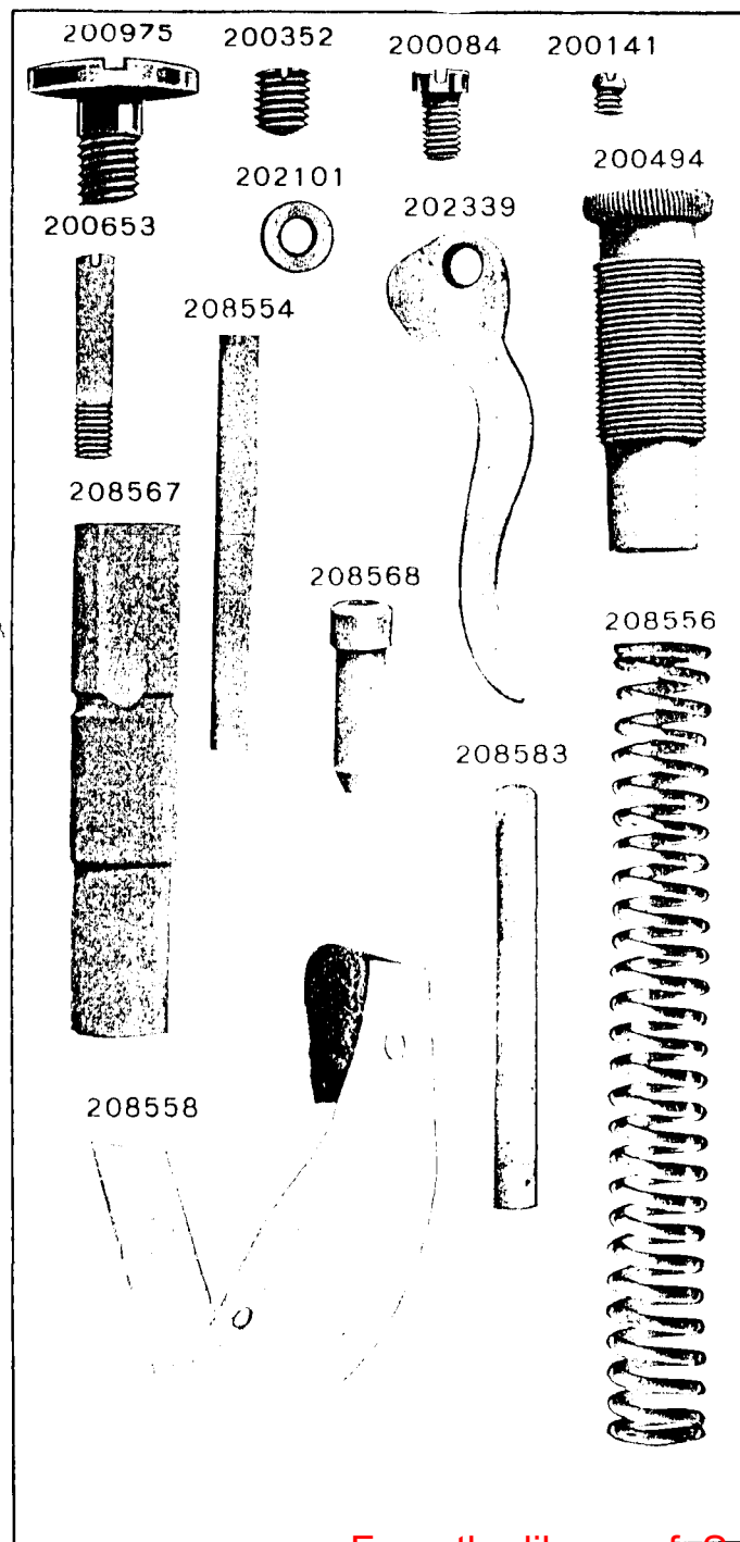
PLATE 11674--FULL SIZE
