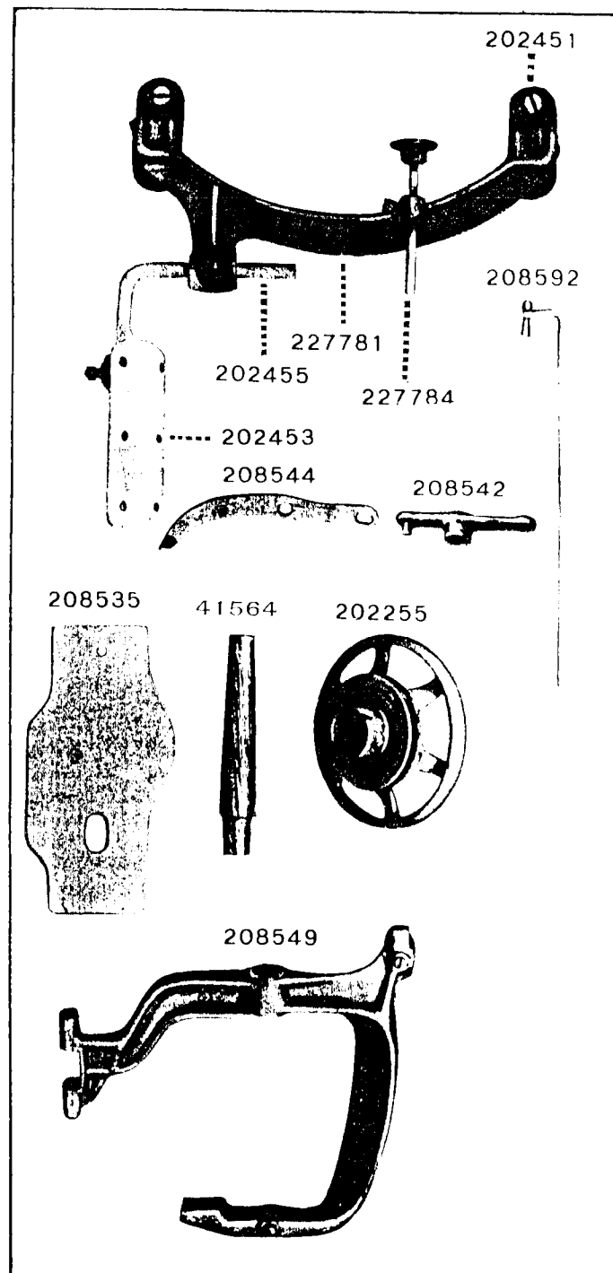
PLATE 11682--ONE-FOURTH SIZE
