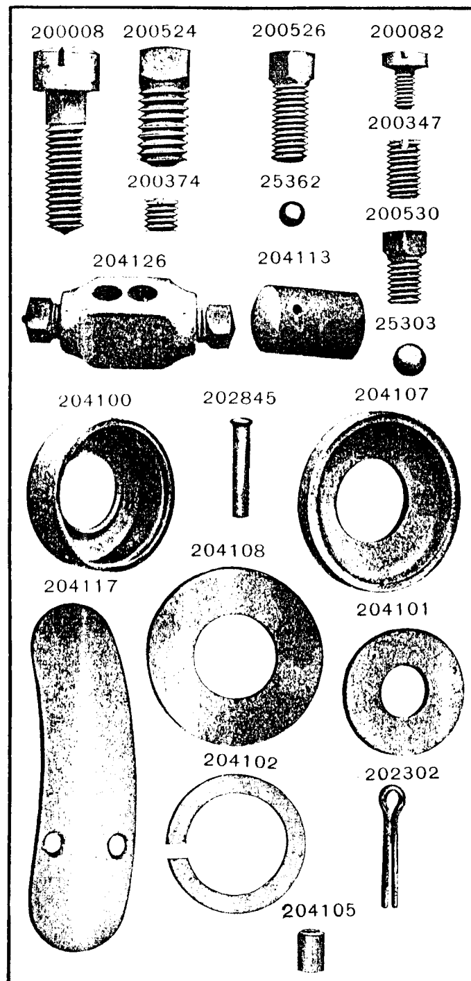
PLATE 12321—FULL SIZE
